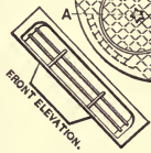
FIG. 6. IRON CURB INLET
